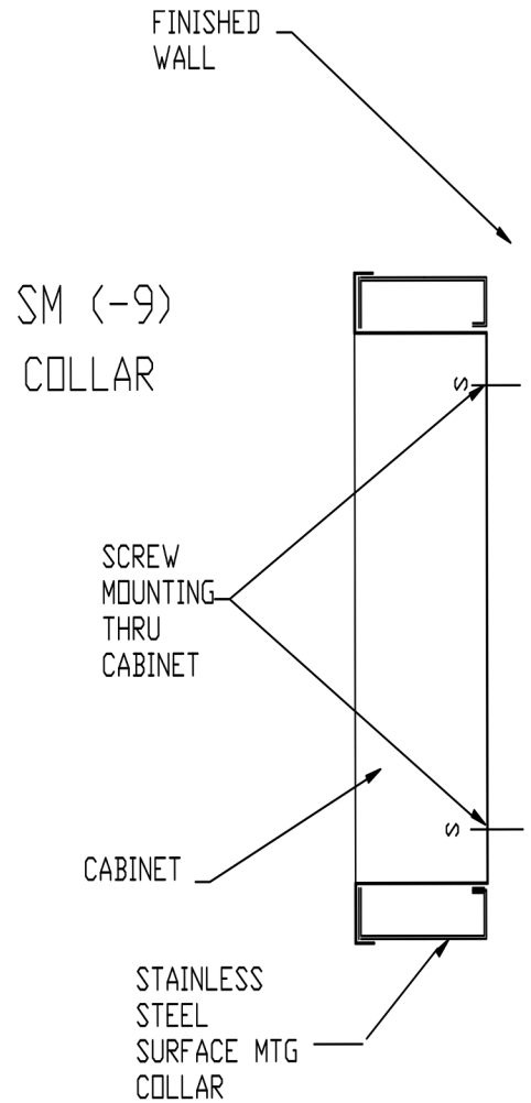
CABINET AND COLLAR ASSEMBLY ARE THEN MOUNTED TO WALL
